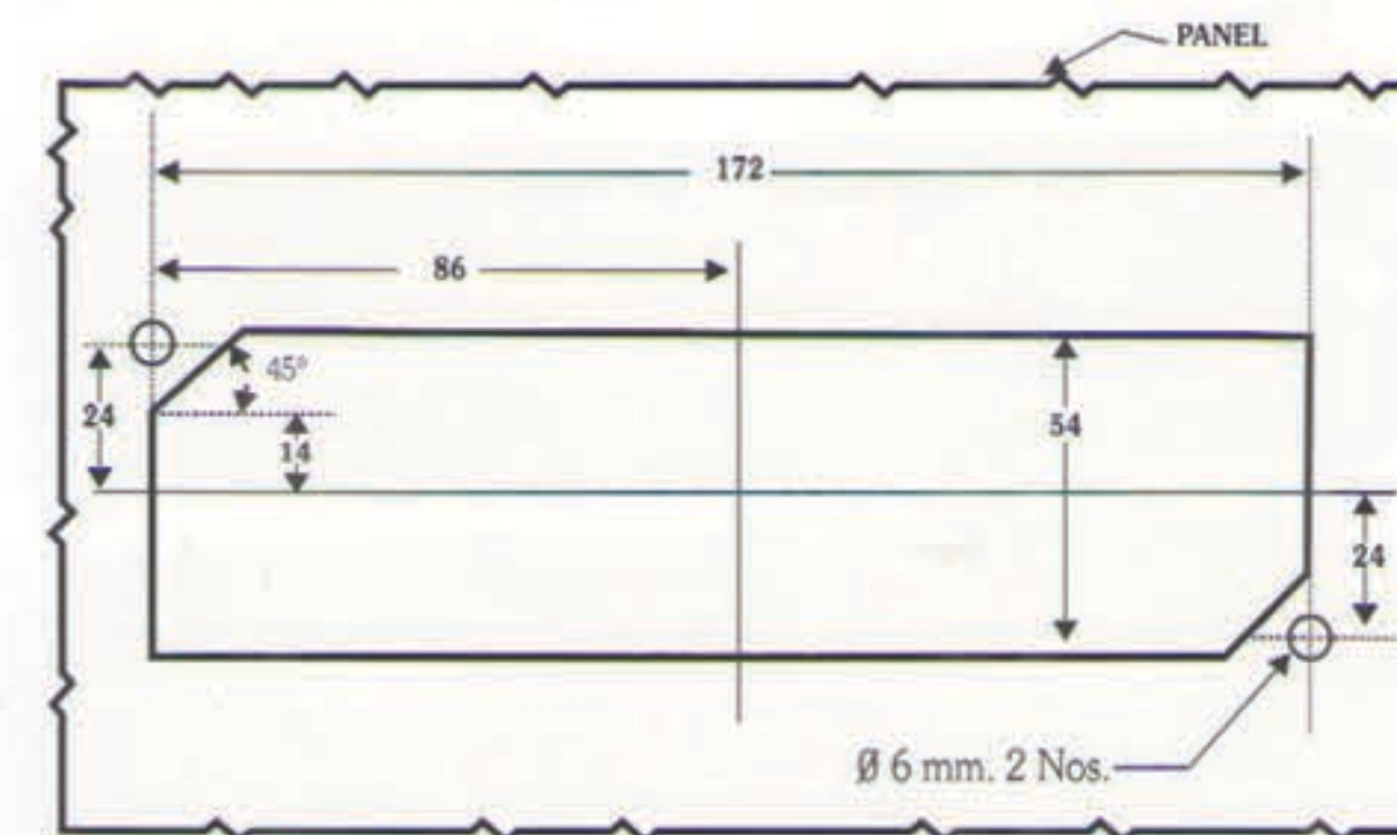
CUTOUT DETAILS FOR 3PH.3WIRE.
