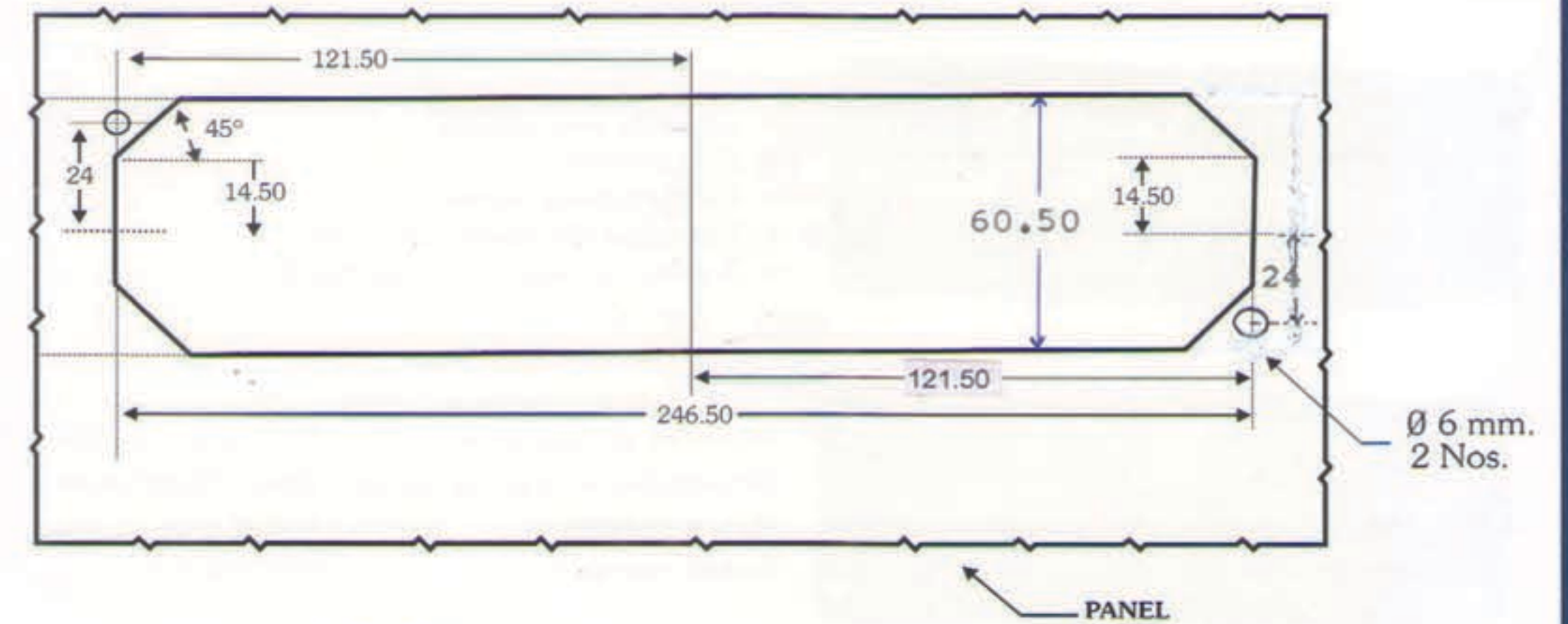
CUTOUT DETAILS FOR 3PH.3WIRE.
